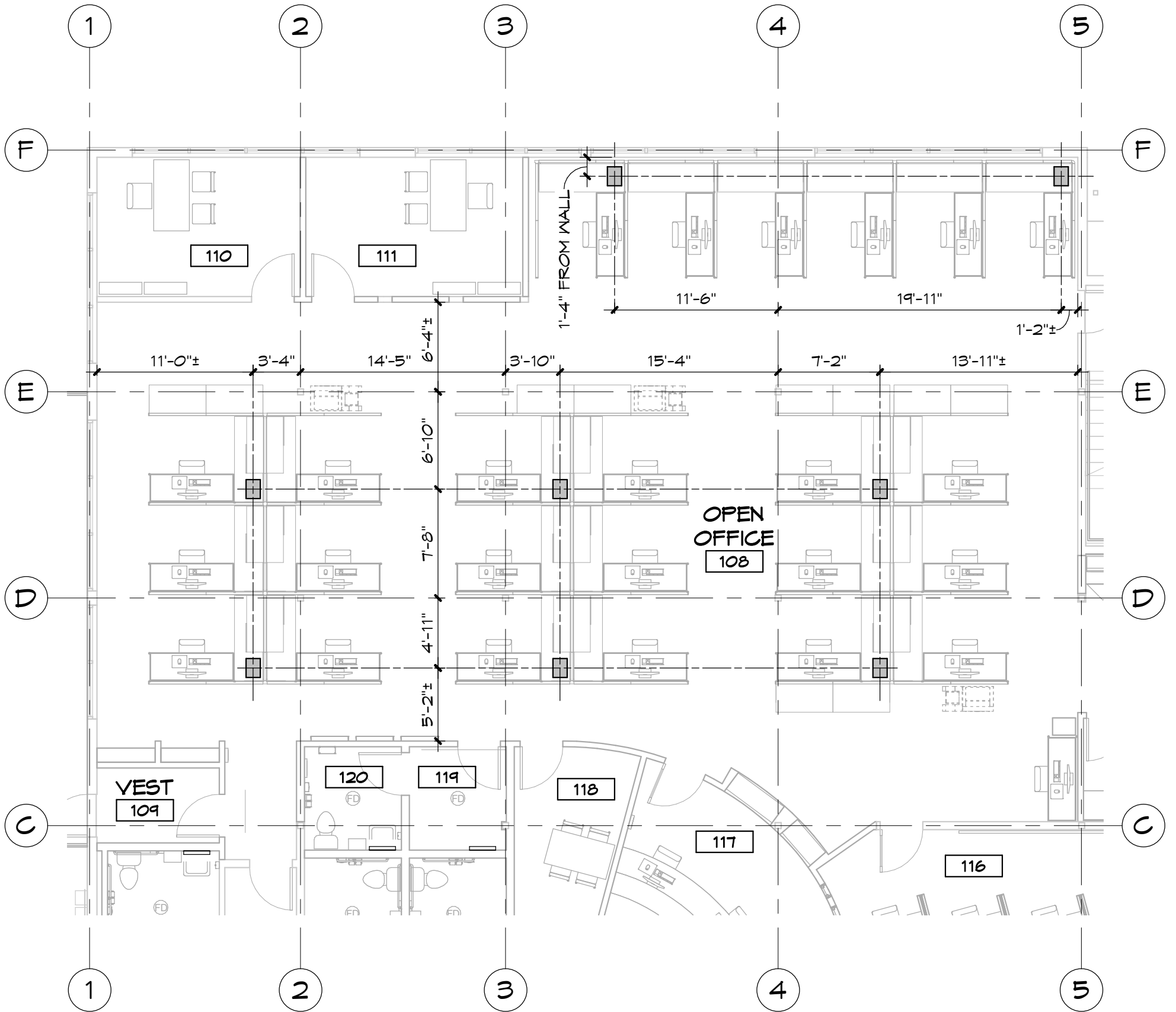
A FIRST FLOOR PLAN - FLOOR BOXES 1/8" = 1'-0"
